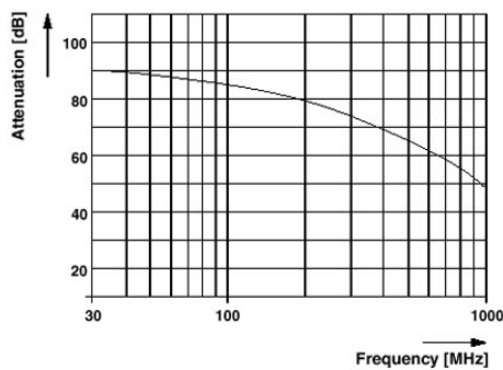
Attenuation curve of the SACC... male/female connectors
