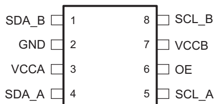
8-PIN SM8 OR US8 (TOP VIEW)
