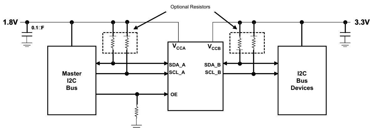
Figure 6. Typical Application Circuit
