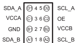
Pin Functions
