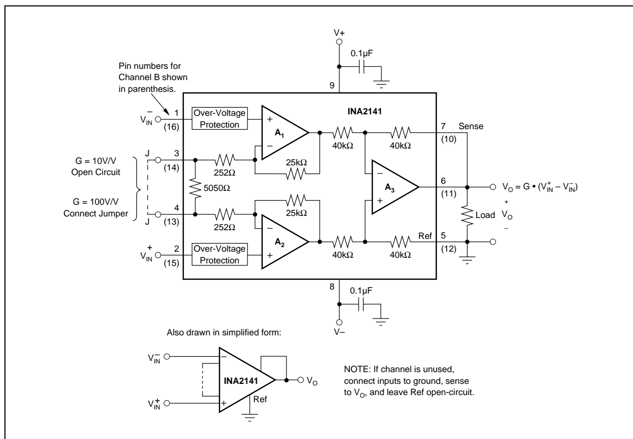
FIGURE 1. Basic Connections.
