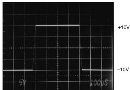
LARGE-SIGNAL RESPONSE, G = 10
