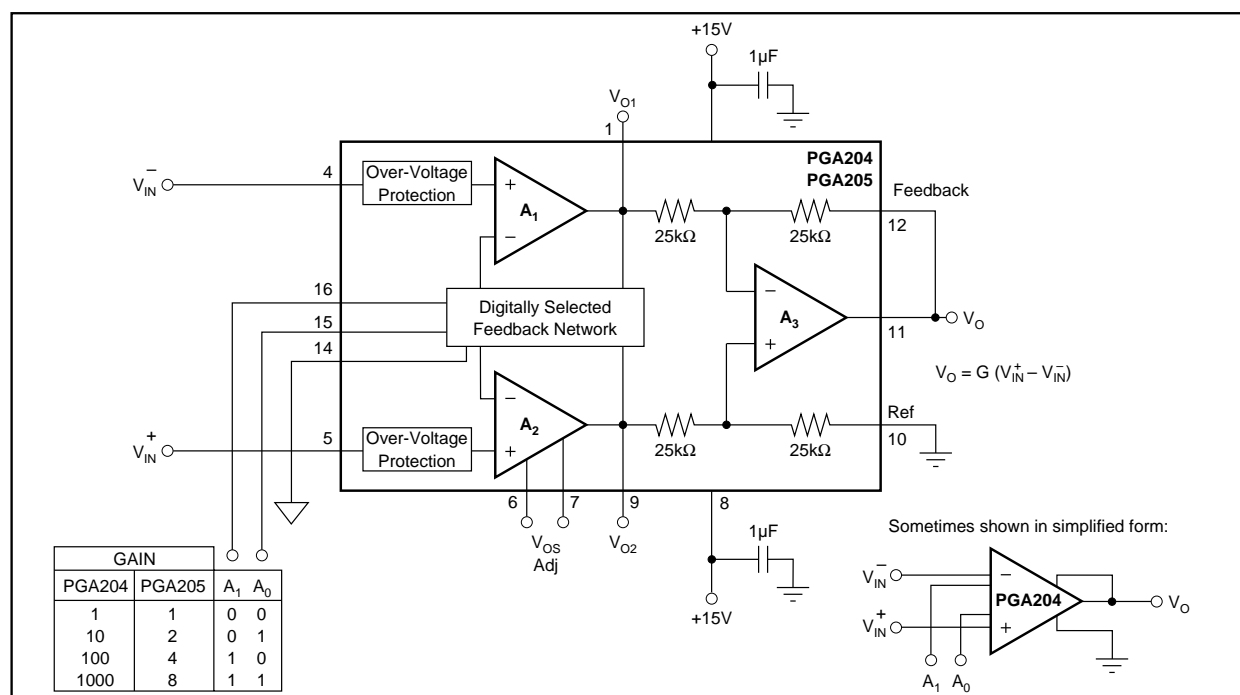
FIGURE 1. Basic Connections.
