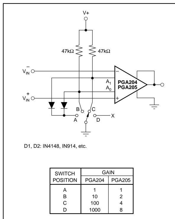
FIGURE 6. Switch-Selected PGIA.
