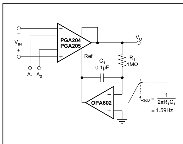
FIGURE 10. AC-Coupled PGIA.
