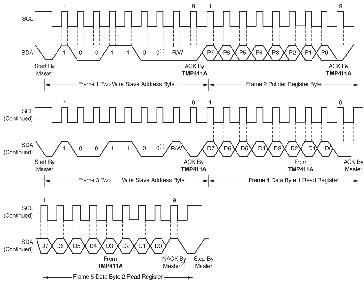
Figure 16. Two-Wire Timing Diagram for Two-Byte Read Format
