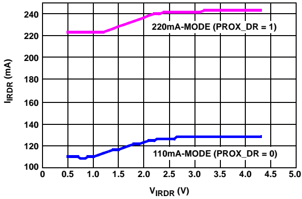
FIGURE 12. IRDR PULSE AMPLITUDE vs V IRDR
