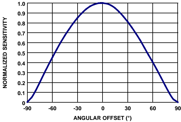
FIGURE 8. ANGULAR SENSITIVITY
