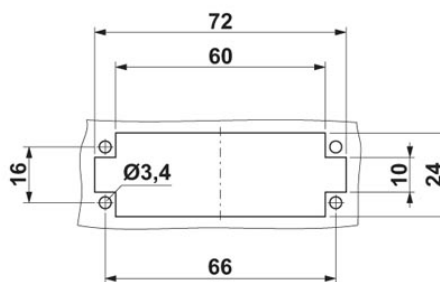
Panel cutout
