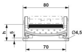
Dimensional drawing
