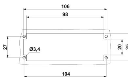
Mounting cut-out
