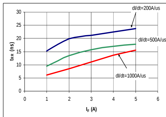
Figure 6. Typical t_{RR} vs I_F at T_J = 125^\circ\text{C}
