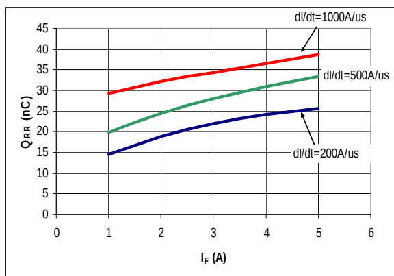
Figure 5. Typical Q_{RR} vs I_F at T_J = 125^\circ\text{C}
