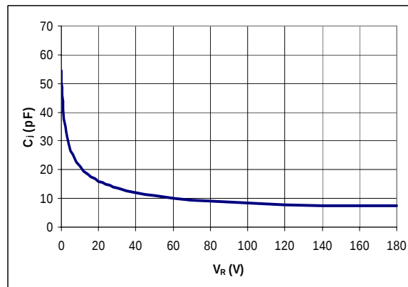
Figure 4. Typical C_j vs V_R
