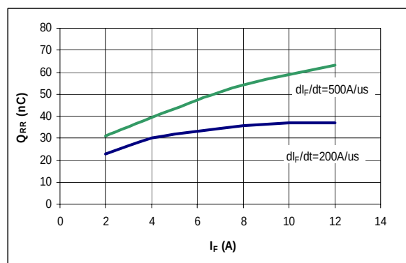
Figure 8. Typical t_{RR} vs I_F at T_J = 125^\circ\text{C}
