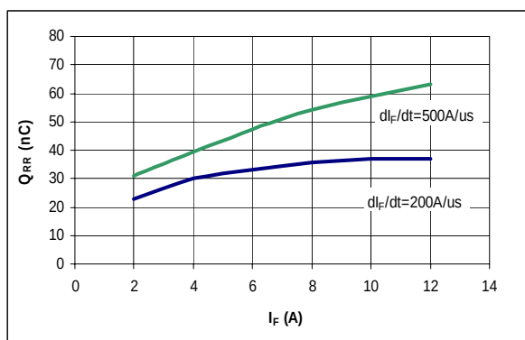
Figure 7. Typical Q_{RR} vs I_F at T_J = 125^\circ\text{C}
