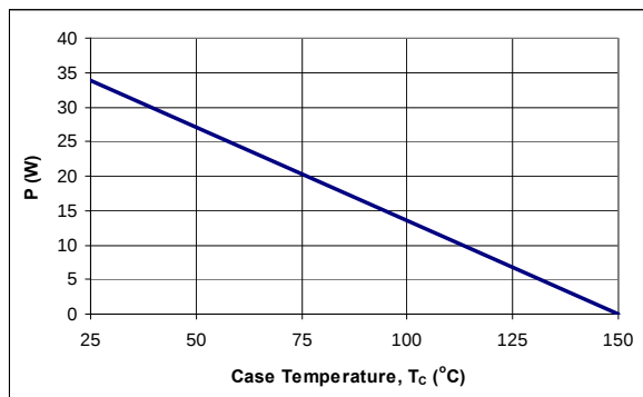
Figure 9. Power Derating Curve
