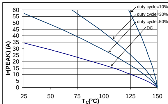
Figure 10. IF(Peak) vs TC, f=70 kHz
