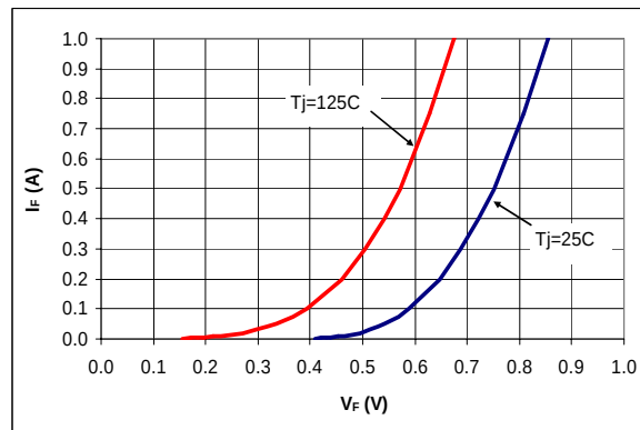
Figure 4. Typical I_F vs V_F
