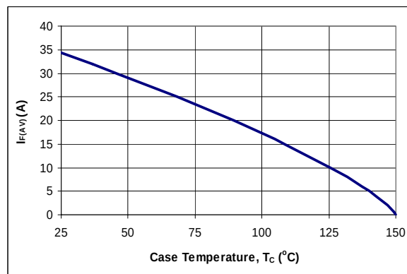
Figure 6. DC Current Derating Curve
