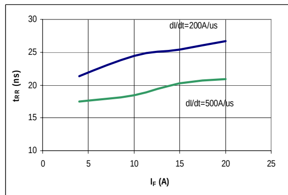
Figure 8. Typical t_{RR} vs I_F at T_J = 125^\circ\text{C}
