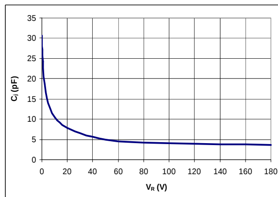
Figure 4. Typical C_i vs V_R
