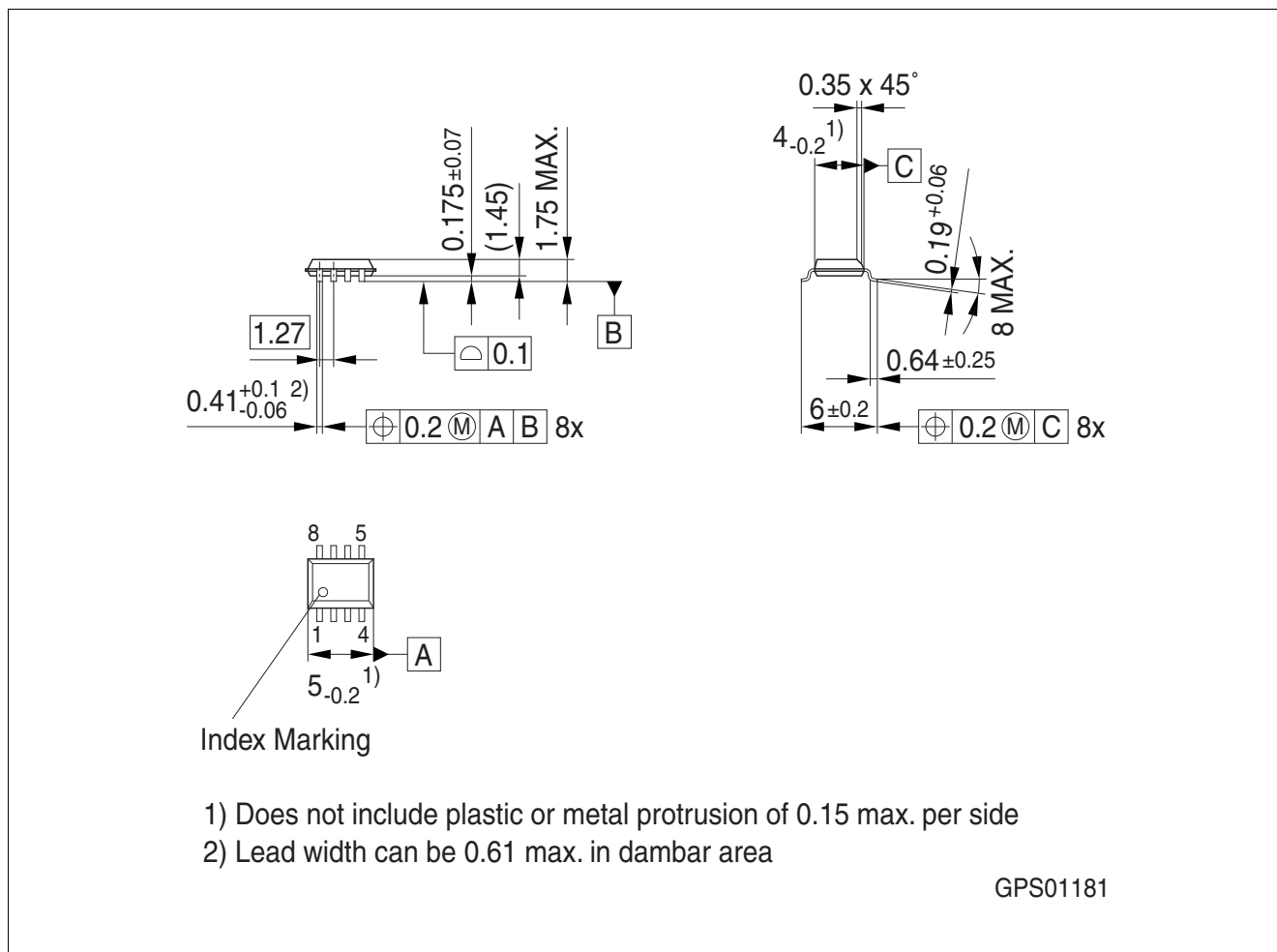
Figure 15 PG-DSO-8 (Plastic Dual Small Outline PG-DSO-8-16)
