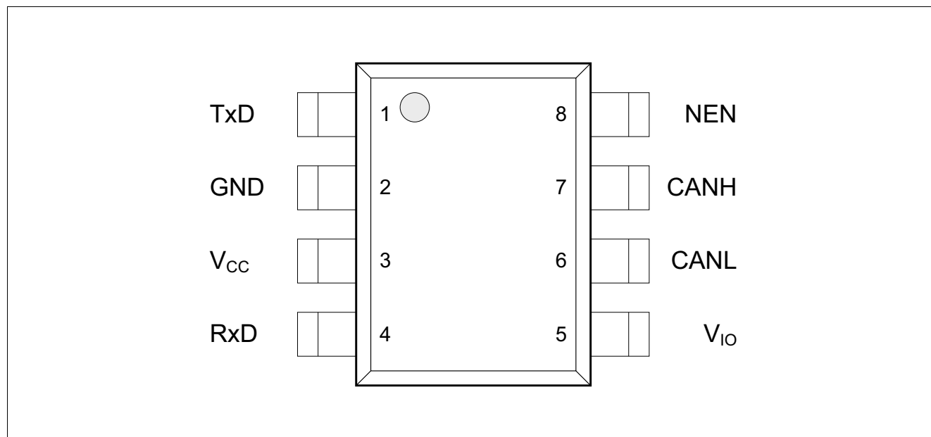
Figure 2 Pin Configuration
