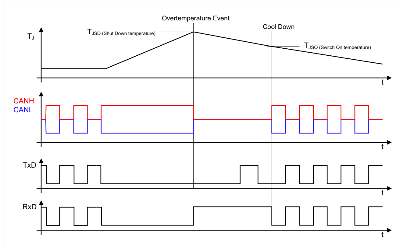
Figure 7 Over-Temperature protection
