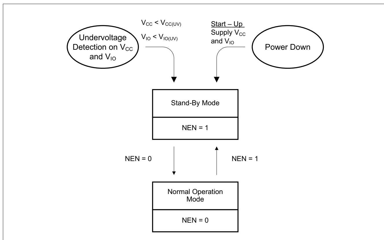
Figure 4 Operation Modes
