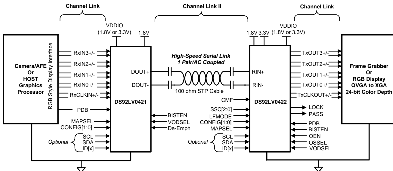
Figure 1. Application Diagram
