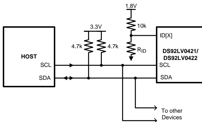
Figure 30. Serial Control Bus Connection
