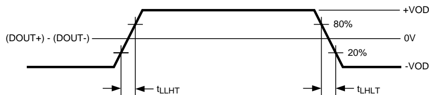
Figure 7. Output Transition Times
