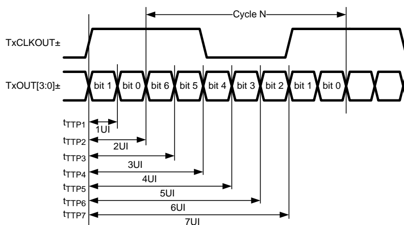
Figure 9. DS92LV0422 LVDS Transmitter Pulse Positions
