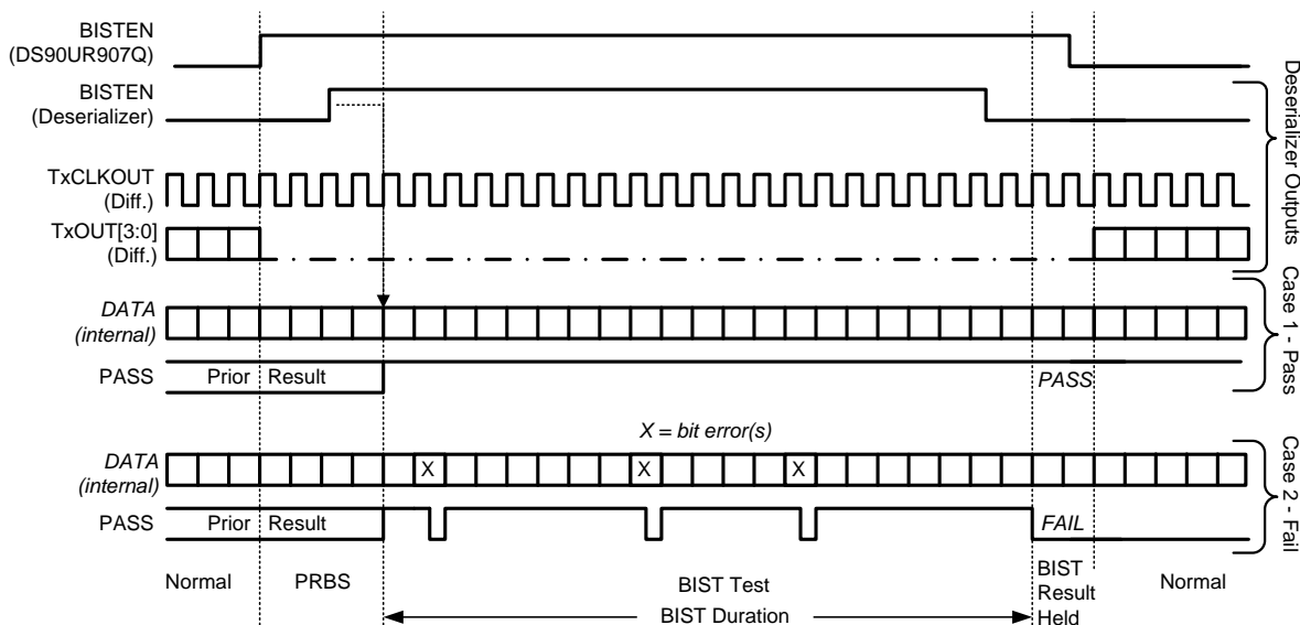
Figure 29. BIST Waveforms
