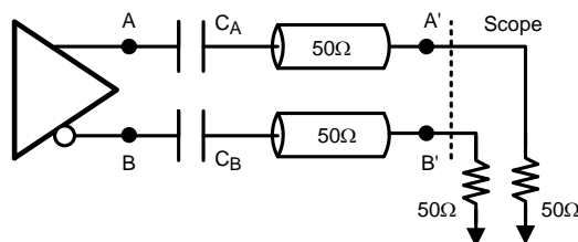
Figure 5. Output Test Circuit
