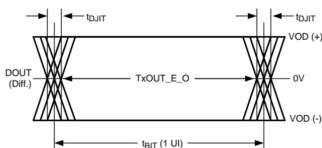
Figure 15. DS92LV0421 Output Jitter
