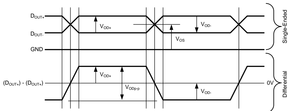
Figure 6. Output Waveforms
