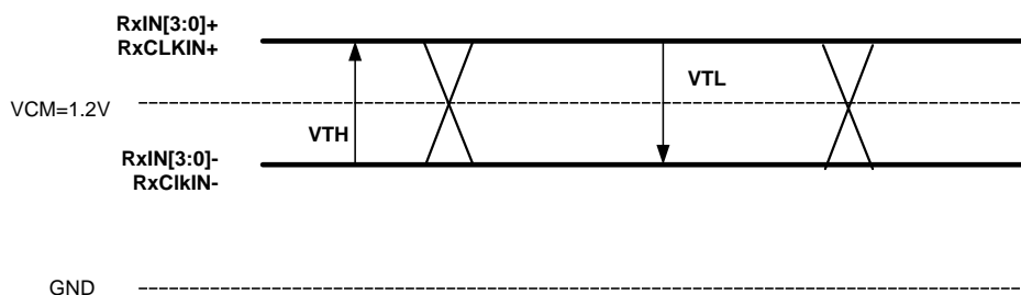
Figure 4. Channel Link DC VTH/VTL Definition
