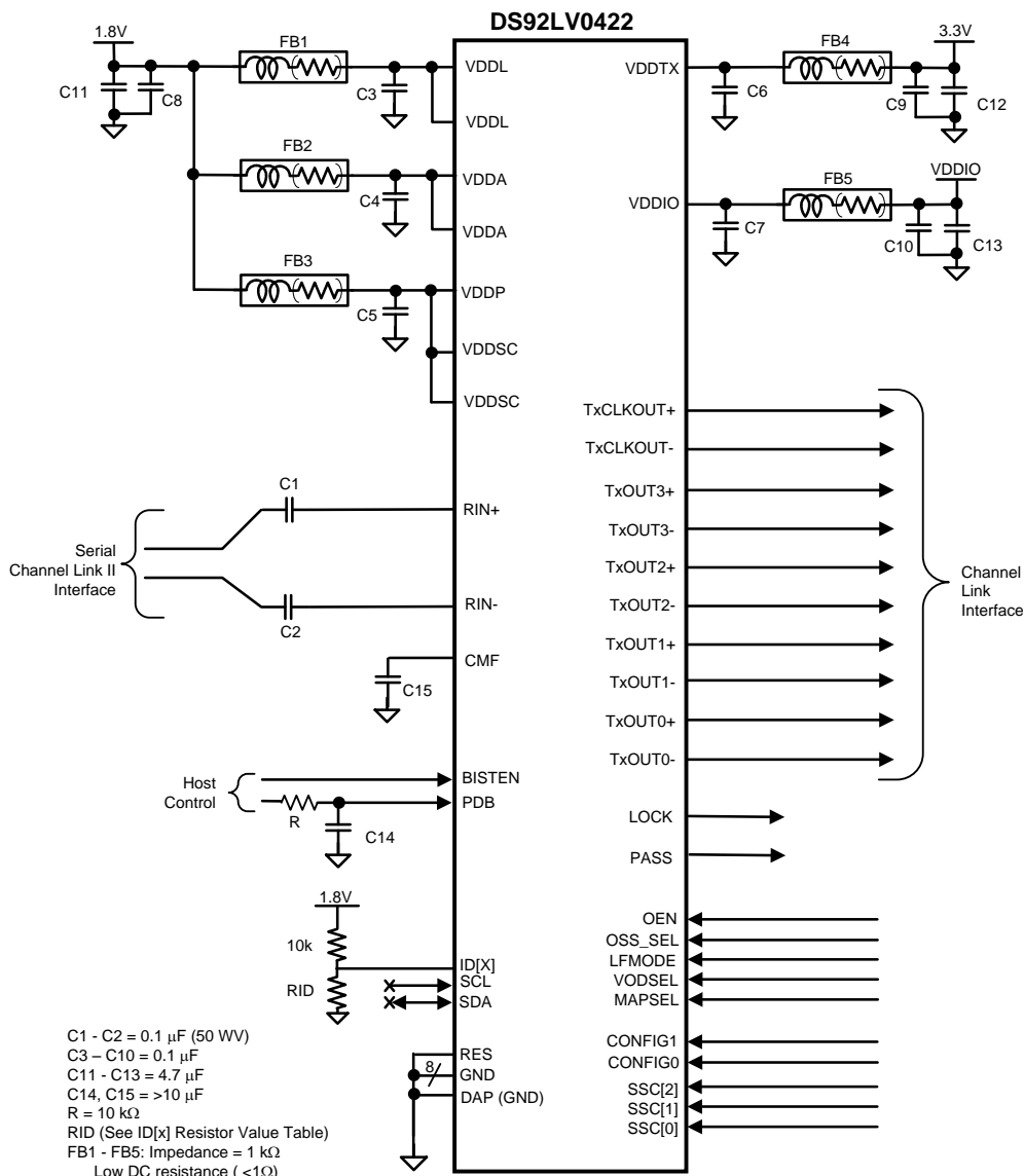
Figure 35. DS92LV0422 Typical Connection Diagram
