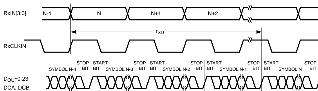
Figure 13. DS92LV0421 Latency Delay
