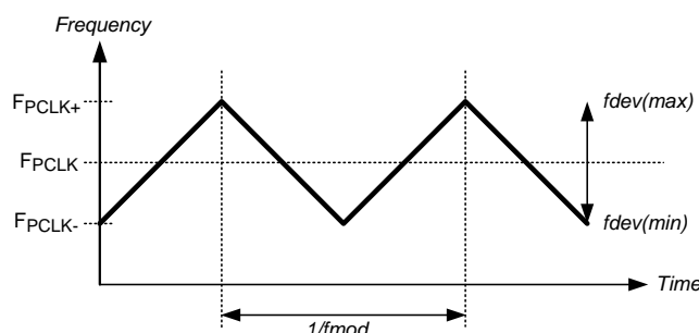
Figure 27. SSCG Waveform
