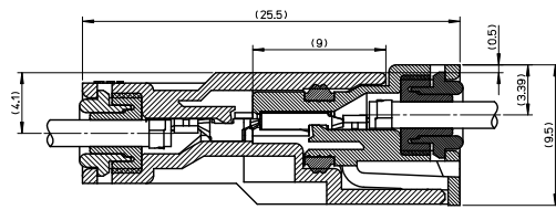
完全状態 FULLY MATED CONDITION
