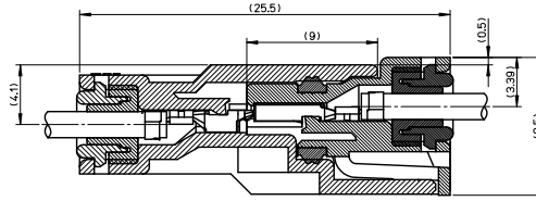
嵌合状態図 FULLY MATED CONDITION
