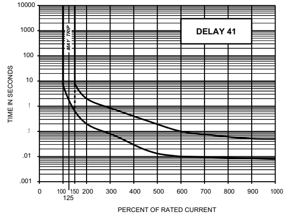
400Hz Delay Curves(typ)
