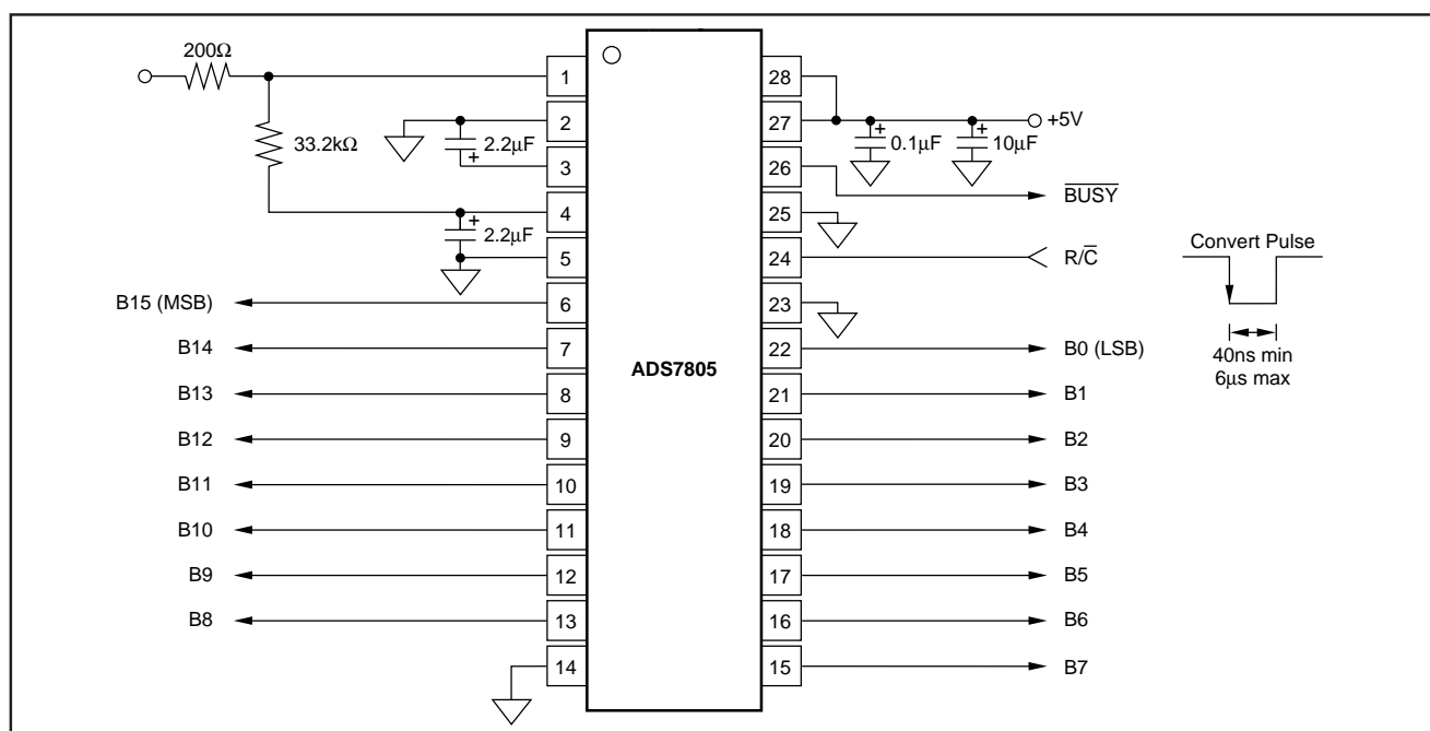
FIGURE 1. Basic Operation.
