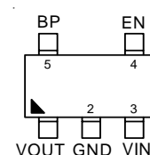
SOT-23-5 (R-Type)
