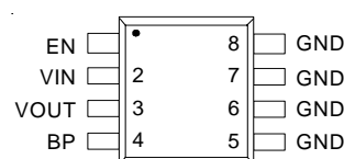
SOP-8
