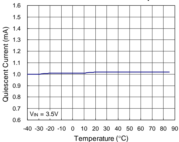
x1 Mode Quiescent Current vs. Temperature
