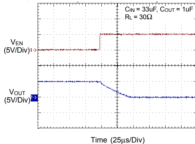
Turn-Off Response
