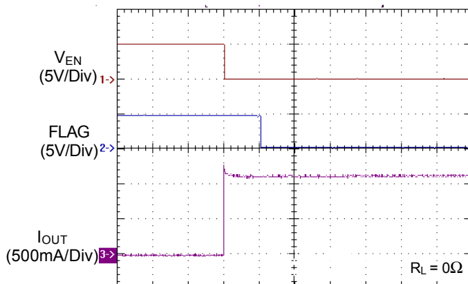
Flag Response with Turn-On Short Current
