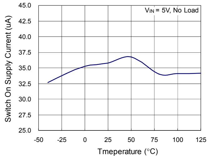
Switch On Supply Current vs. Temperature
