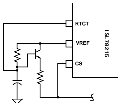
FIGURE 7. SLOPE COMPENSATION
