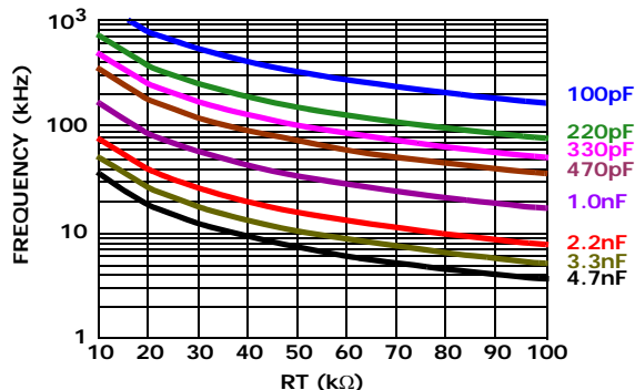
FIGURE 4. RESISTANCE FOR CT CAPACITOR VALUES GIVEN
