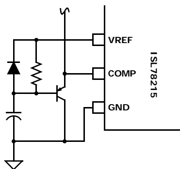
FIGURE 5. SOFT-START
