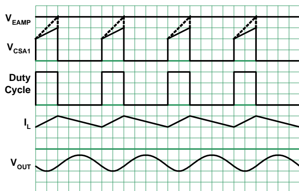
FIGURE 66. PWM OPERATION WAVEFORMS
