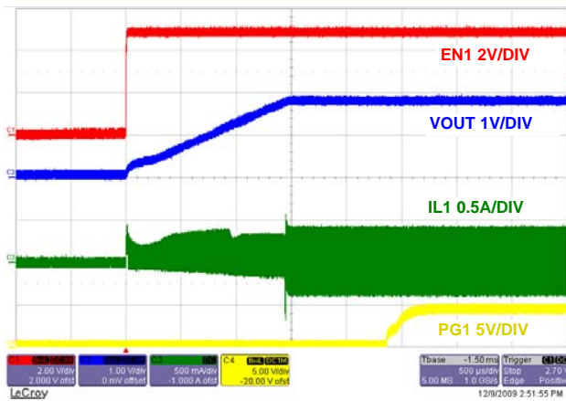
FIGURE 15. SOFT-START WITH NO LOAD CHANNEL 1
