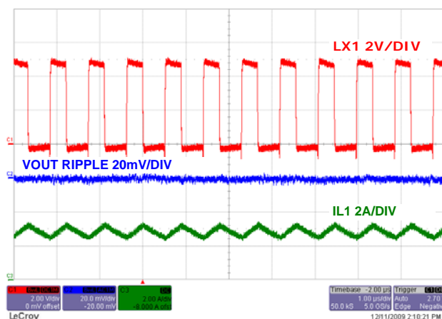
FIGURE 11. STEADY STATE OPERATION WITH FULL LOAD CHANNEL 1
