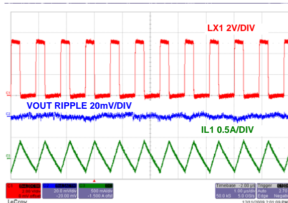
FIGURE 49. STEADY STATE OPERATION AT NO LOAD CHANNEL 1
