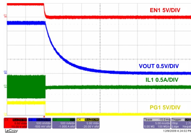
FIGURE 57. SOFT-DISCHARGE SHUTDOWN CHANNEL 1
