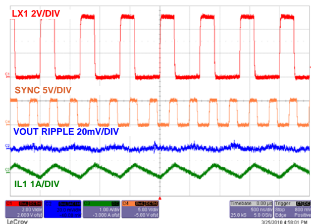
FIGURE 58. STEADY STATE OPERATION CH1 AT NO LOAD WITH F_{SW} = 3MHz
