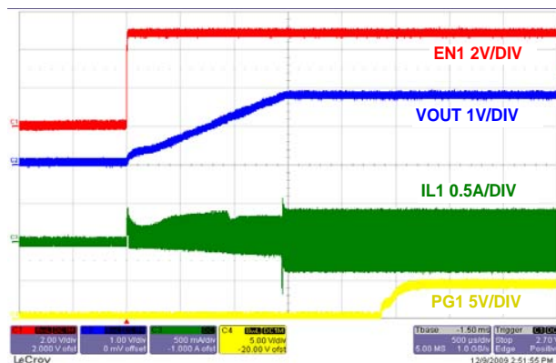
FIGURE 55. SOFT-START WITH NO LOAD CHANNEL 1
