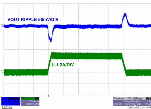
FIGURE 13. LOAD TRANSIENT CHANNEL 1
