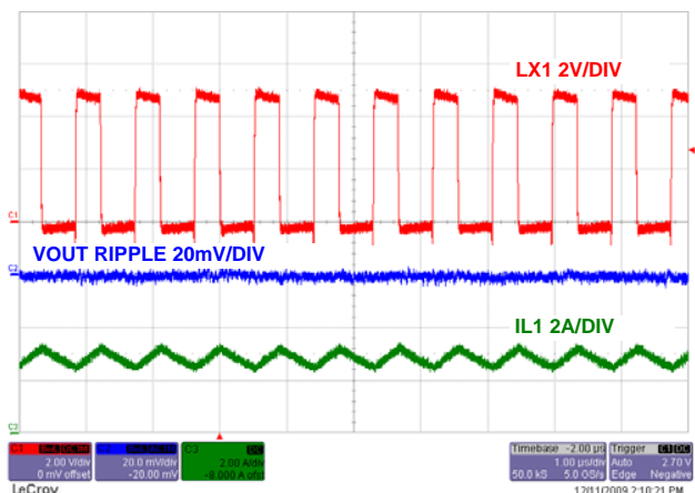
FIGURE 50. STEADY STATE OPERATION WITH FULL LOAD CHANNEL 1
