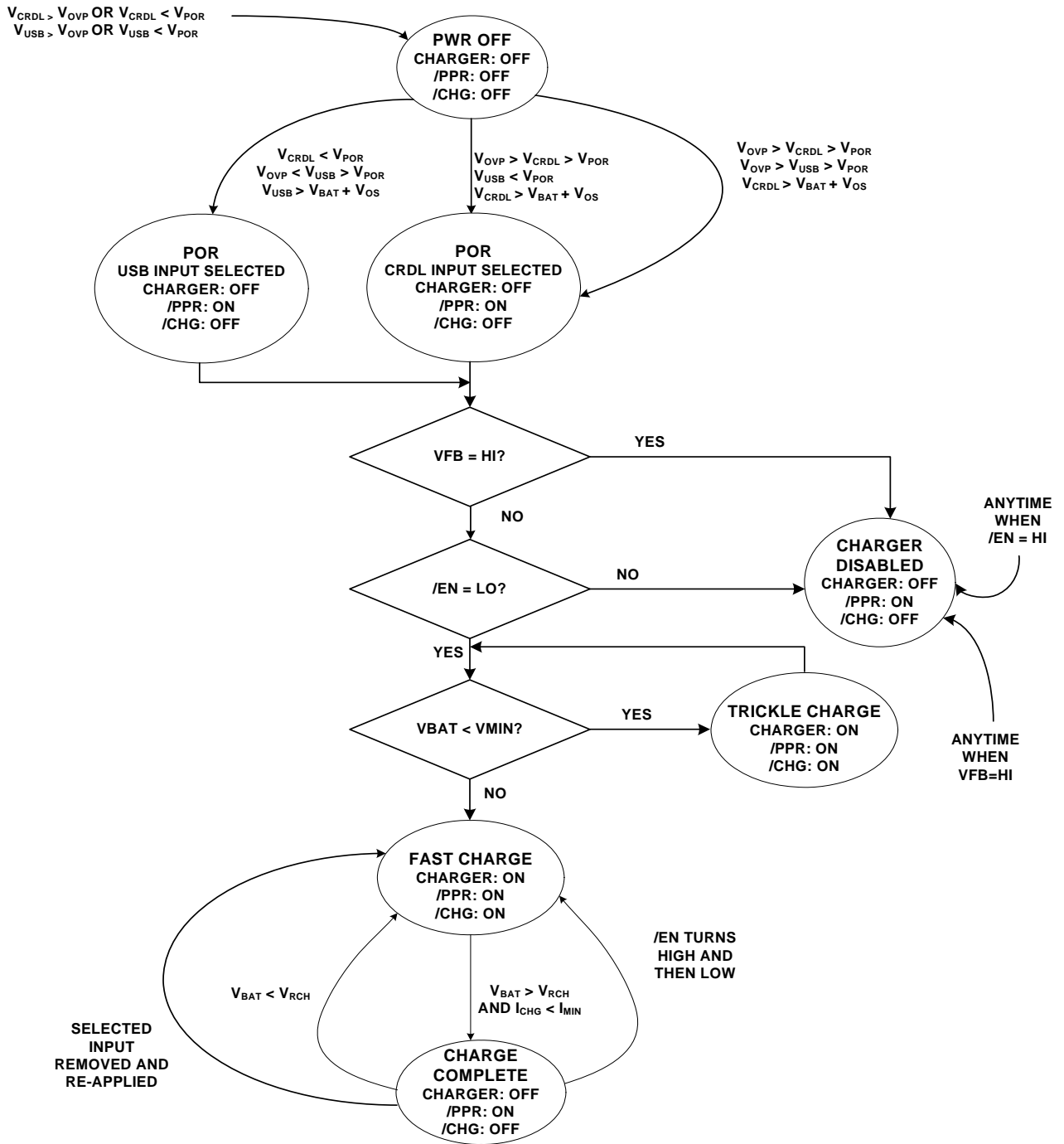
FIGURE 12. STATE DIAGRAM
