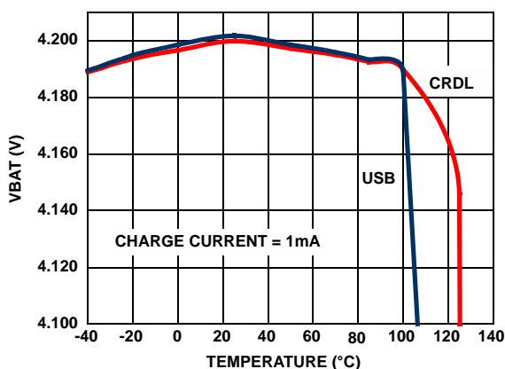
FIGURE 1. CHARGER OUTPUT VOLTAGE vs TEMPERATURE
