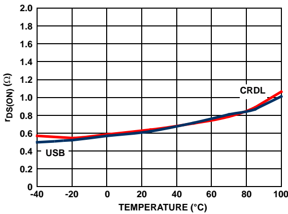
FIGURE 5. r_{DS(ON)} vs TEMPERATURE AT 3.7V OUTPUT
