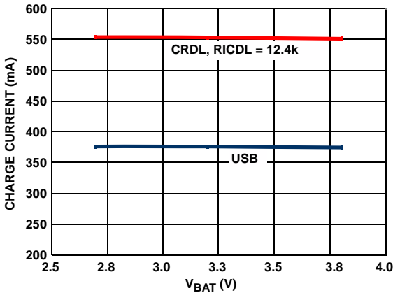
FIGURE 3. CHARGE CURRENT vs OUTPUT VOLTAGE
