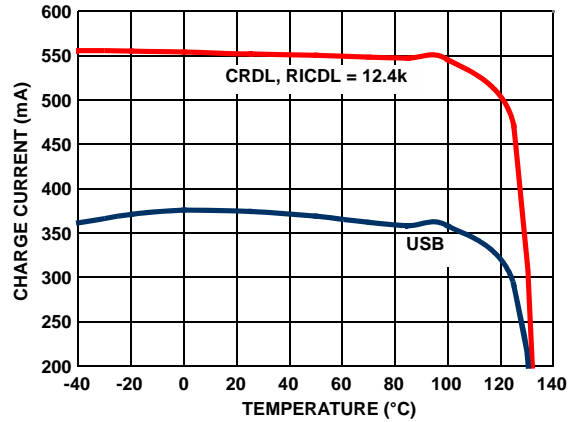
FIGURE 4. CHARGE CURRENT vs AMBIENT TEMPERATURE
