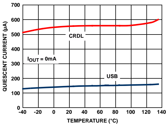
FIGURE 7. CRADLE INPUT QUIESCENT CURRENT vs TEMPERATURE
