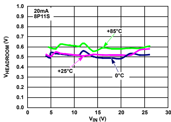
FIGURE 13. V_{HEADROOM} vs V_{IN} vs TEMPERATURE AT 20mA
