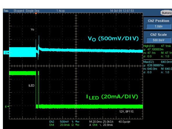
FIGURE 23. LOAD REGULATION WITH I_{LED} CHANGES FROM 100% TO 0% PWM DIMMING
