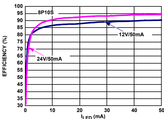
FIGURE 6. EFFICIENCY vs I_{LED}
