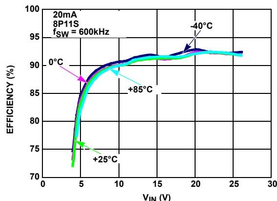
FIGURE 5. EFFICIENCY vs V_{IN} vs TEMPERATURE AT 20mA
