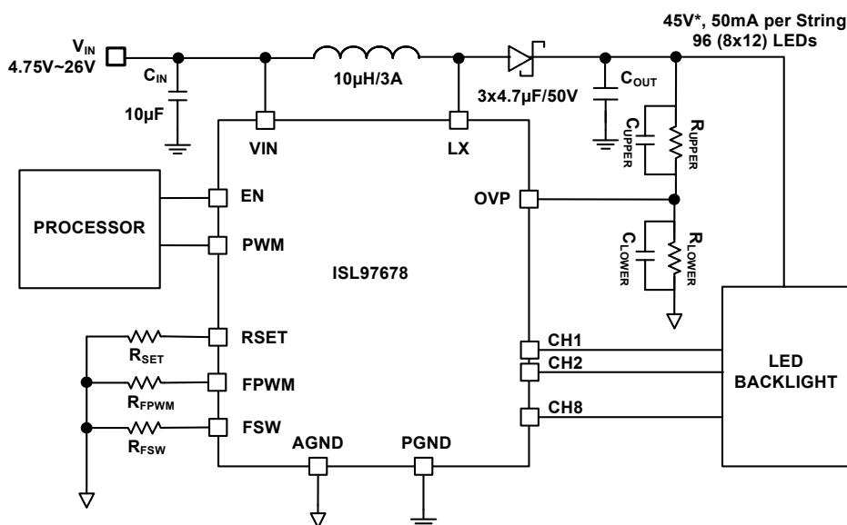
FIGURE 1. TYPICAL APPLICATION CIRCUIT: TFT-LCD NOTEBOOK DISPLAY
