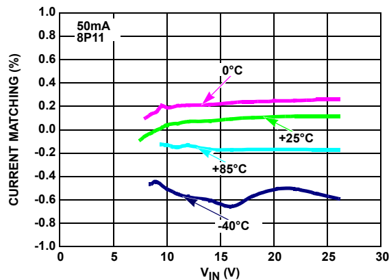
FIGURE 9. CURRENT MATCHING vs V_{IN} vs TEMPERATURE
