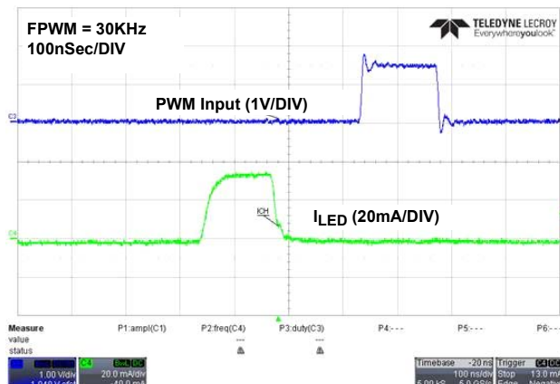
FIGURE 25. MINIMUM 0.4% PWM DIMMING DUTY CYCLE
