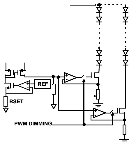
FIGURE 26. SIMPLIFIED CURRENT SOURCE CIRCUIT
