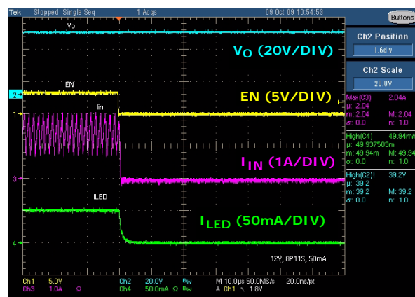
FIGURE 24. DISABLE PROFILE
