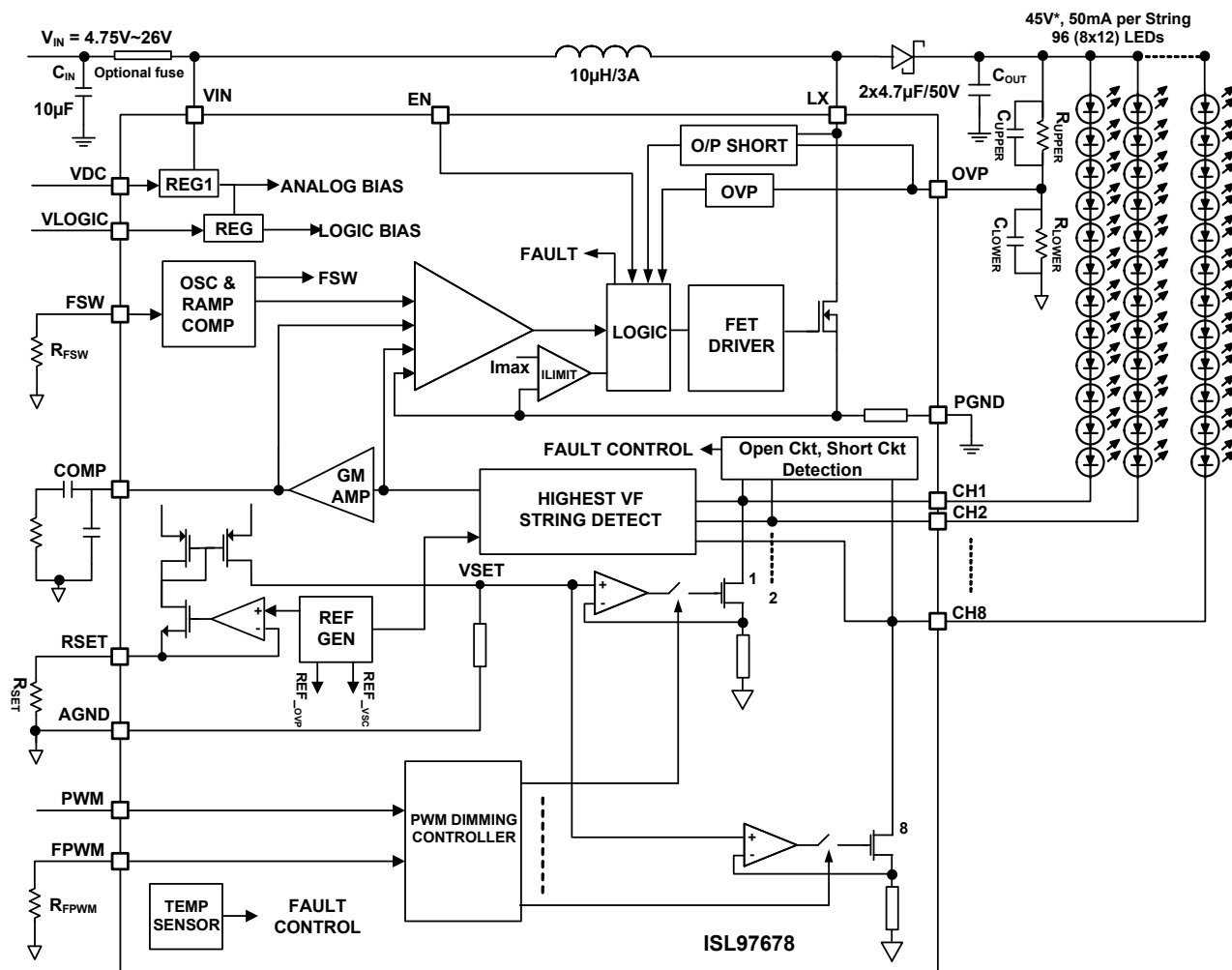
FIGURE 3. ISL97678 BLOCK DIAGRAM
