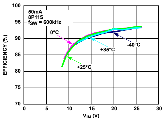
FIGURE 4. EFFICIENCY vs V_{IN} vs TEMPERATURE AT 50mA
