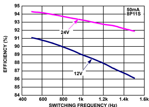
FIGURE 7. EFFICIENCY vs SWITCHING FREQUENCY
