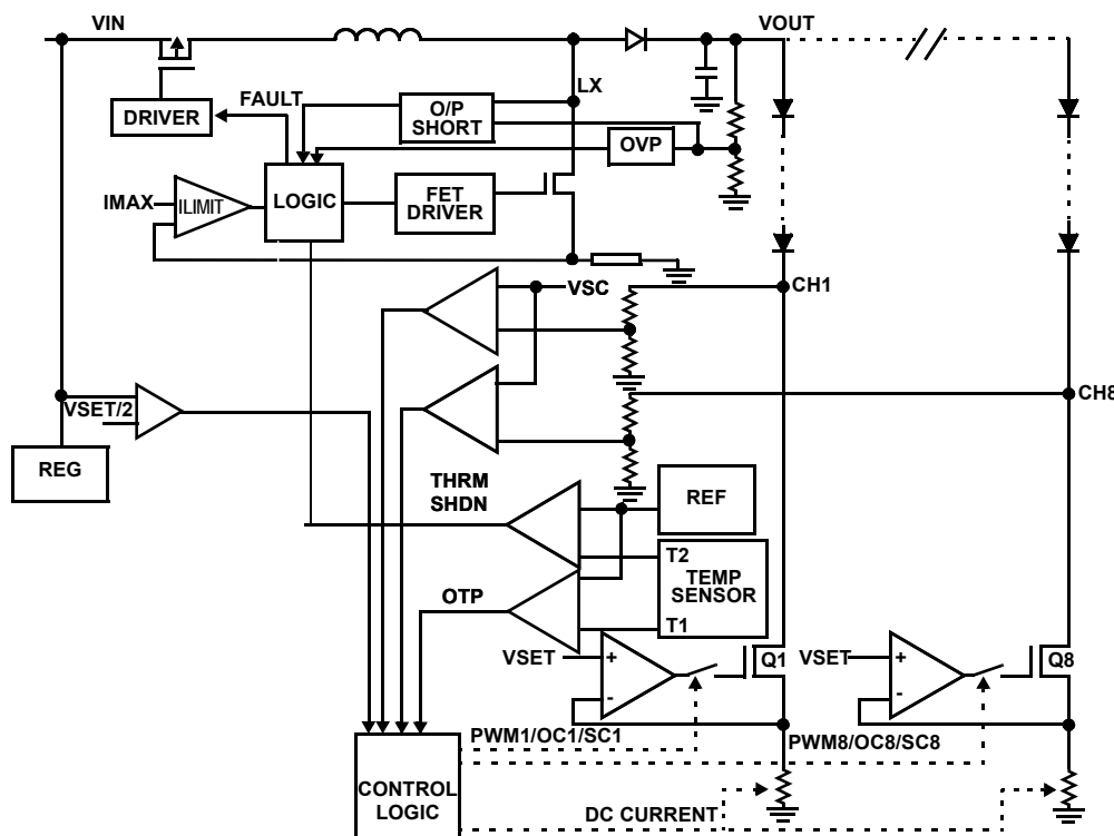
FIGURE 27. SIMPLIFIED FAULT PROTECTIONS
