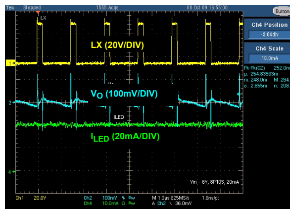
FIGURE 15. V_{OUT} RIPPAGE VOLTAGE
