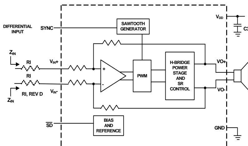
FIGURE 21. TYPICAL CIRCUIT WITH DIFFERENTIAL INPUT
