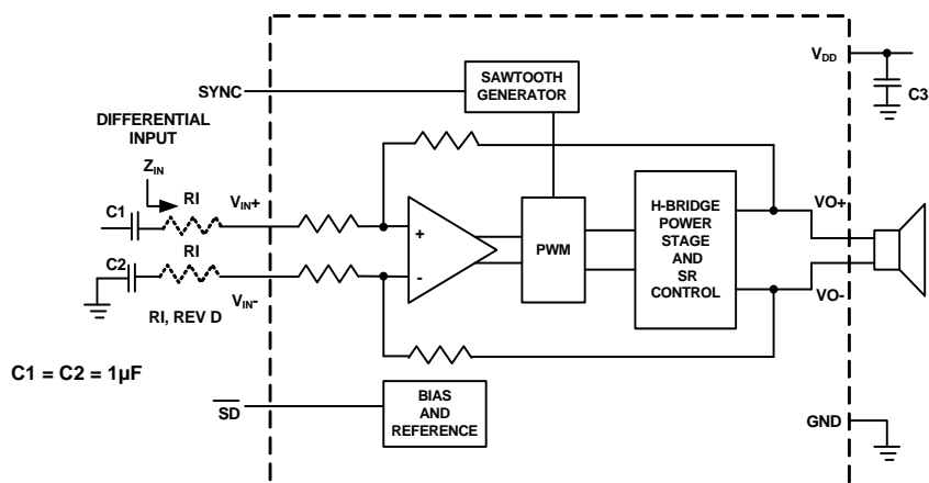
FIGURE 23. TYPICAL CIRCUIT WITH SINGLE-ENDED INPUT
