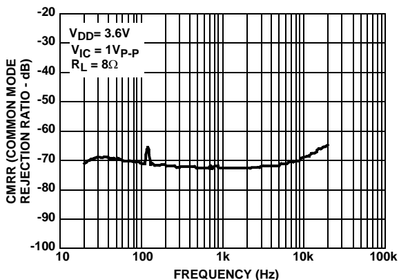
FIGURE 5. COMMON MODE REJECTION MODE vs FREQUENCY
