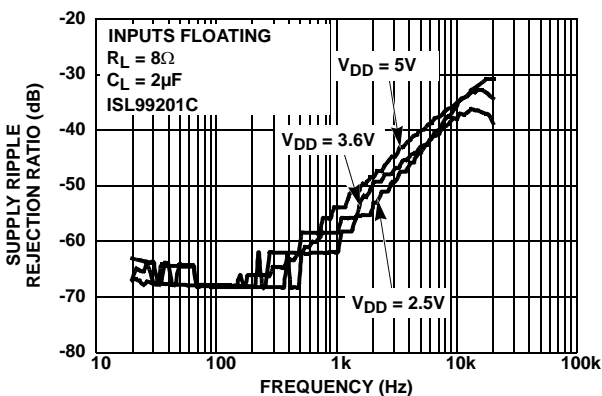
FIGURE 17. SUPPLY RIPPLE REJECTION RATIO vs FREQUENCY - ISL99201C
