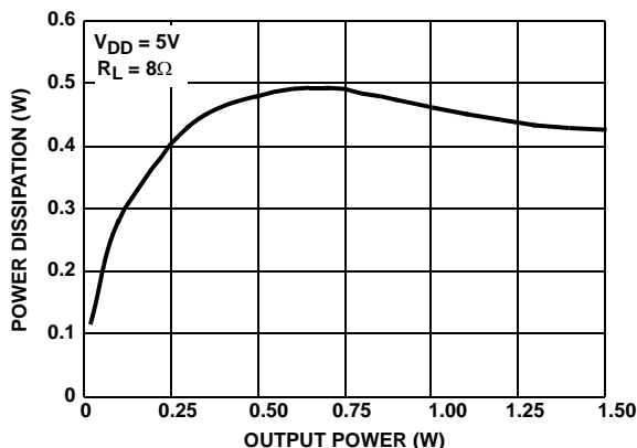
FIGURE 7. POWER DISSIPATION vs OUTPUT POWER
