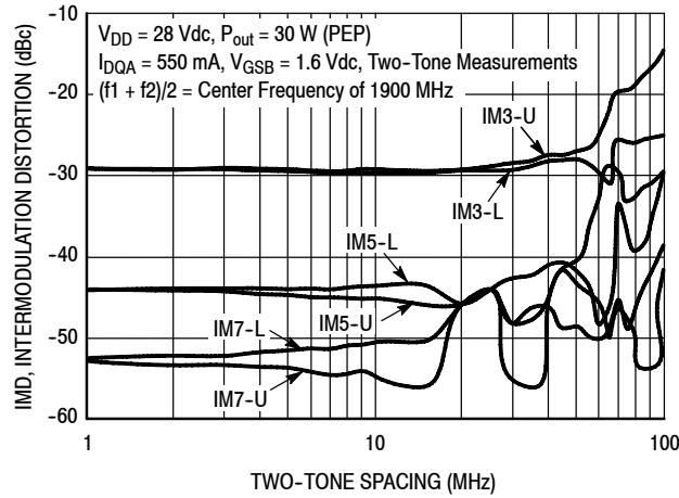
Figure 5. Intermodulation Distortion Products versus Two-Tone Spacing
