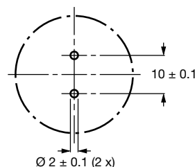
Fig. 3 - Mounting hole diagram
