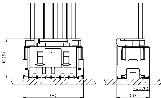
嵌合図 MATED CONNECTORS
