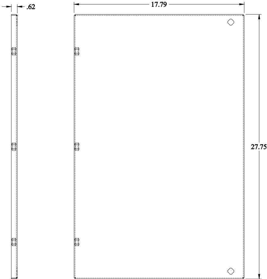
SIDE VIEW
