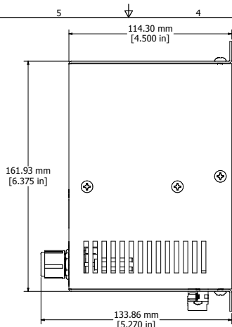
ASSEMBLY - VIEW FROM SIDE
