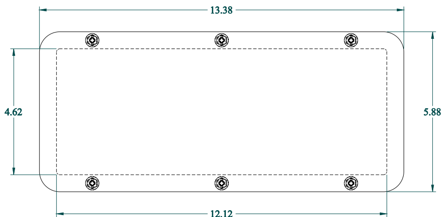
FRONT VIEW
