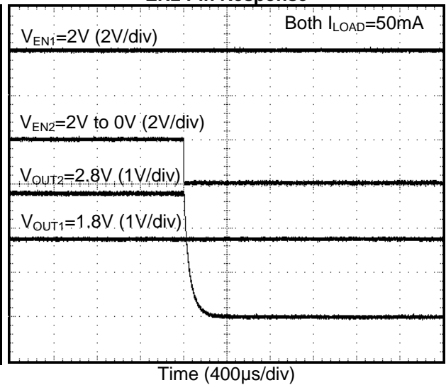
EN2 Pin Response
