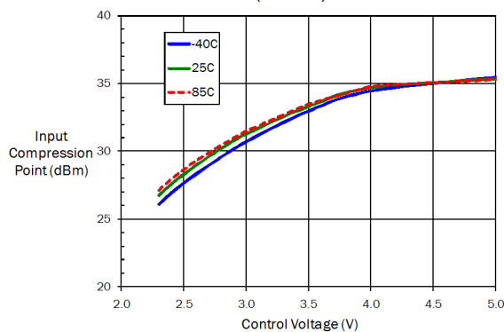
P1dB Compression Point versus Control Voltage (915MHz)
