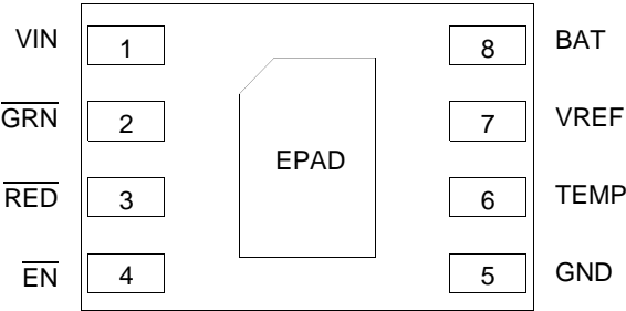
Figure 3. 34674 Pin Connections
