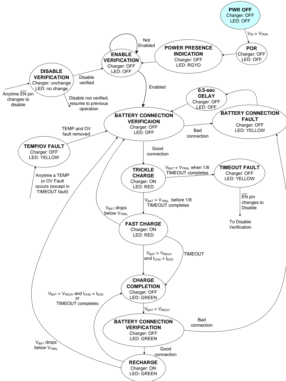
Figure 23. 34674 Flow Chart
