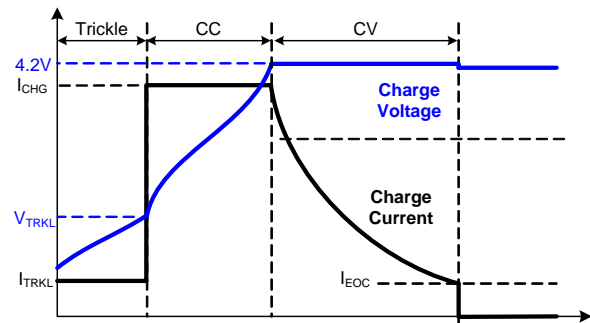
Figure 17. Charge Profile
