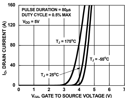
Figure 7. Transfer Characteristics
