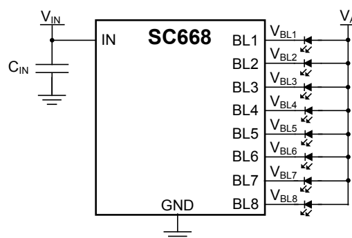
Figure 1 — Anode Supply
