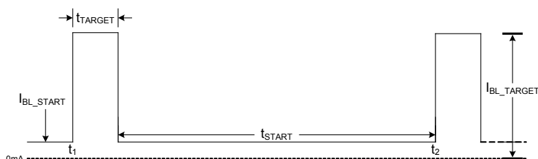
Figure 4 — Blink Timing Diagram
