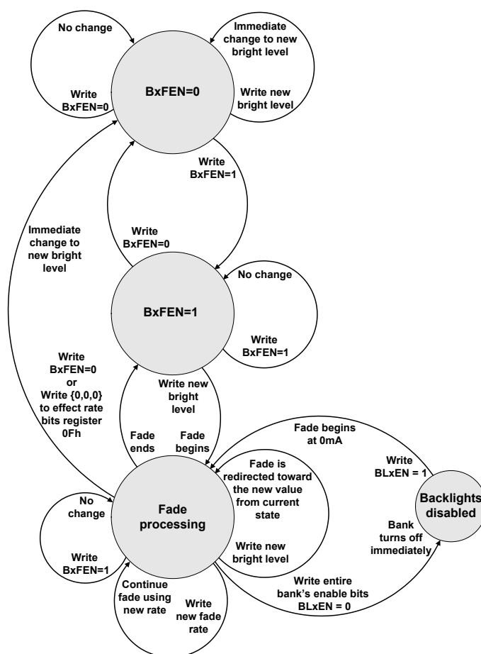
Figure 2 — State Diagram for Fade Function
