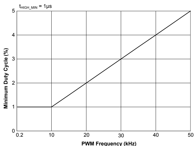
Figure 9 — Minimum Duty Cycle
