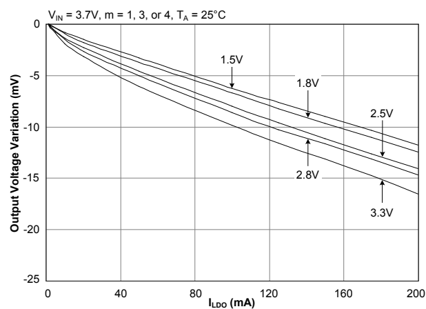
Load Regulation (LDOm)
