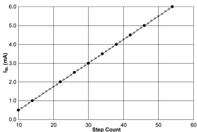
Figure 11 — Backlight Steps (0.5mA to 6.0mA)
