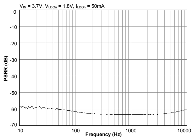
PSRR vs. Frequency (1.8V)
