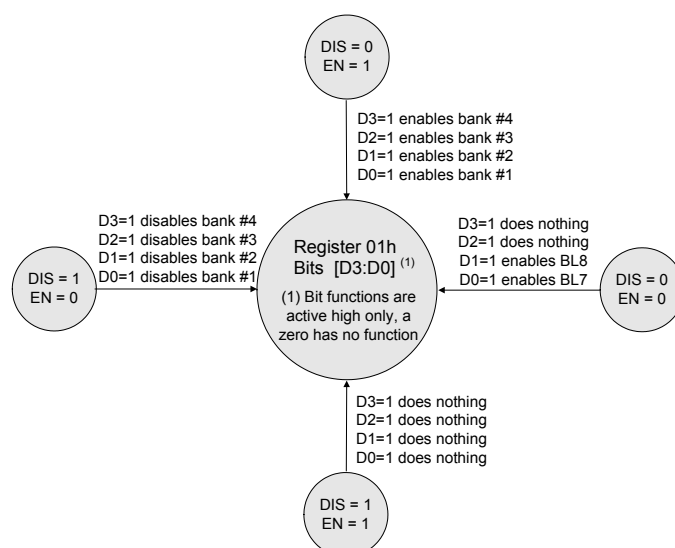
Figure 19 — Multi-function Bits of Register (01h)
