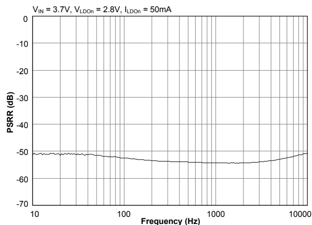
PSRR vs. Frequency (2.8V)
