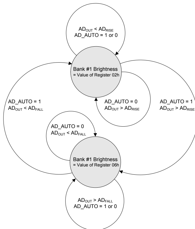
Figure 29 — ADC function at Bank #1 Brightness
