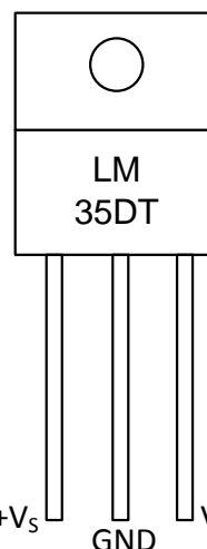
NEB Package 3-Pin TO-220 (Top View)
