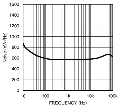
Figure 10. Noise Voltage
