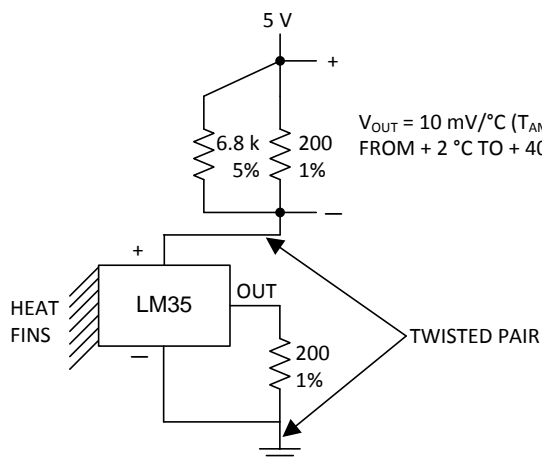
Figure 16. Two-Wire Remote Temperature Sensor (Grounded Sensor)
