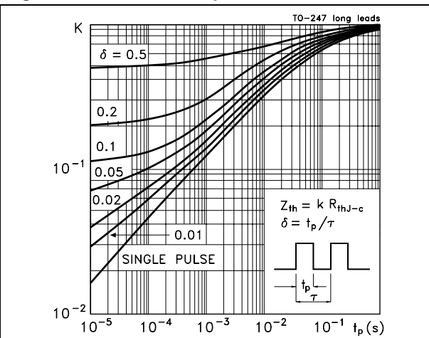
Figure 15. Thermal impedance
