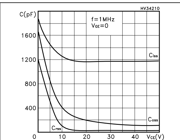
Figure 7. Capacitance variations
