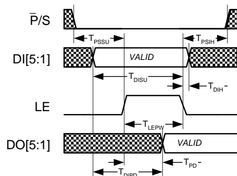
Figure 16. Latched-Parallel/Direct-Parallel Timing Diagram
