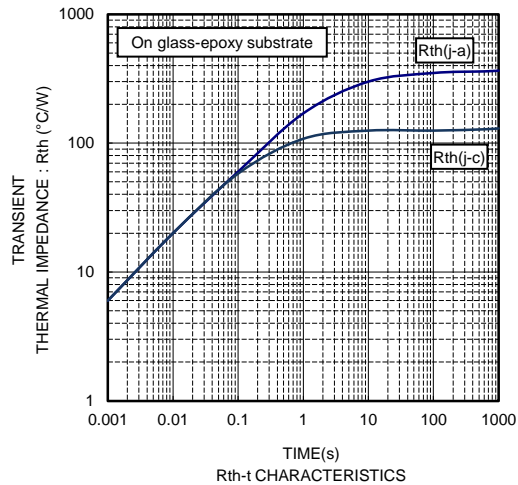
Rth-t CHARACTERISTICS
