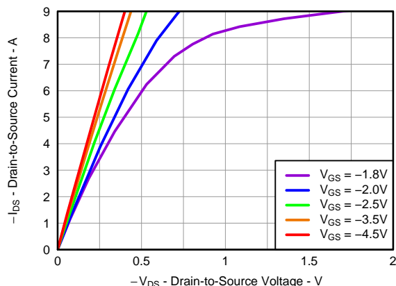
Figure 2. Saturation Characteristics
