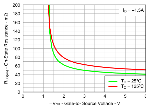
Figure 7. On Resistance vs. Gate Voltage
