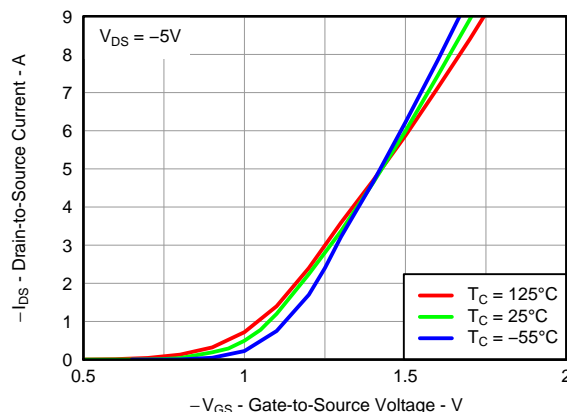
Figure 3. Transfer Characteristics
