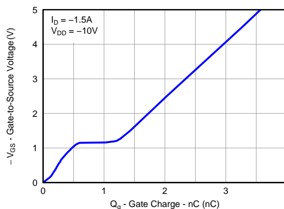
Gate Charge
