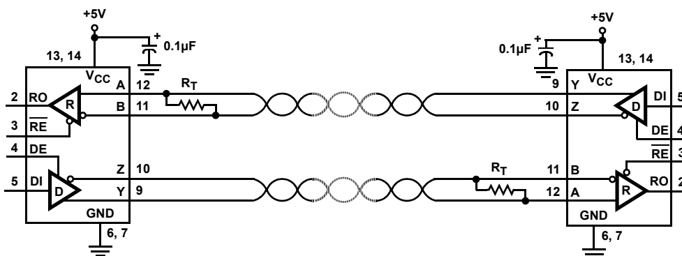
ISL32470E FULL DUPLEX EXAMPLE
