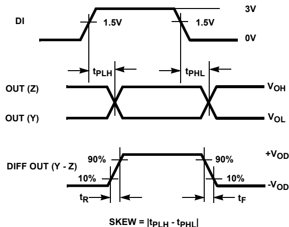
FIGURE 4B. MEASUREMENT POINTS
