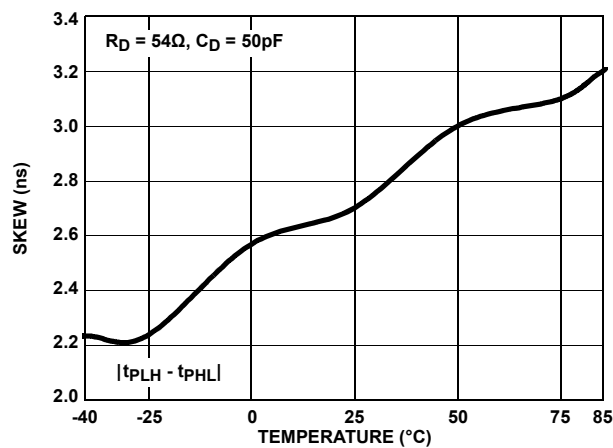
FIGURE 21. DRIVER DIFFERENTIAL SKEW vs TEMPERATURE (ISL32478E)
