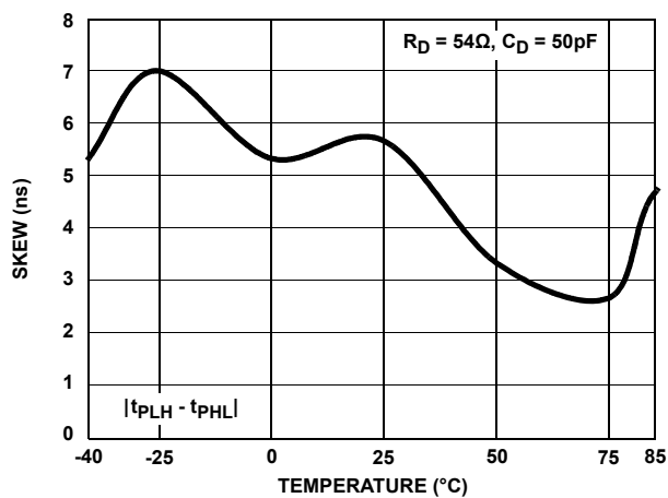
FIGURE 17. DRIVER DIFFERENTIAL SKEW vs TEMPERATURE (ISL32470E, ISL32472E)
