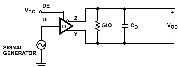
FIGURE 6A. TEST CIRCUIT
