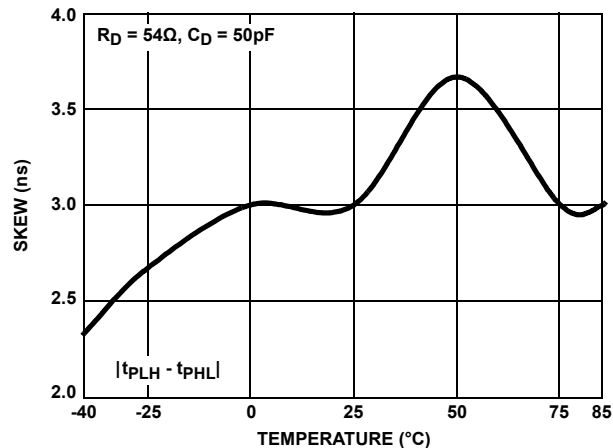
FIGURE 19. DRIVER DIFFERENTIAL SKEW vs TEMPERATURE (ISL32475E)
