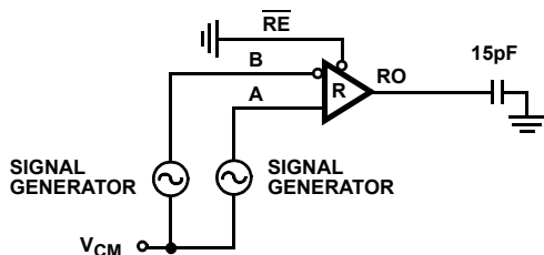
FIGURE 7A. TEST CIRCUIT
