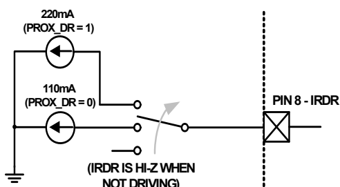
FIGURE 5. CURRENT DRIVE MODE OPTIONS
