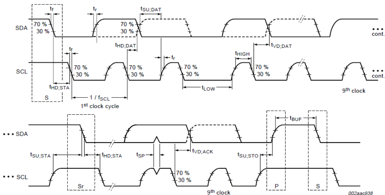
FIGURE 2. I²C TIMING DIAGRAM
