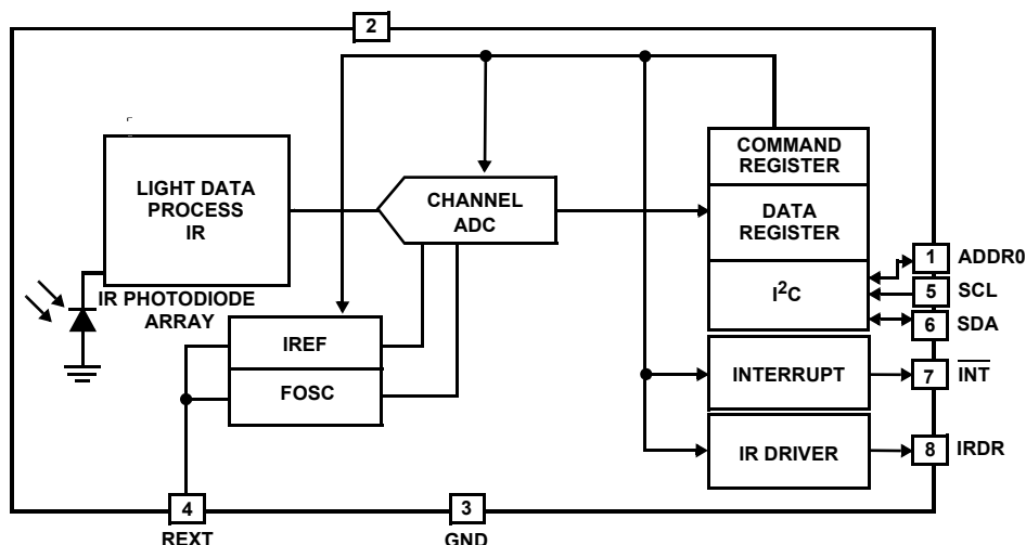
FIGURE 1. BLOCK DIAGRAM
