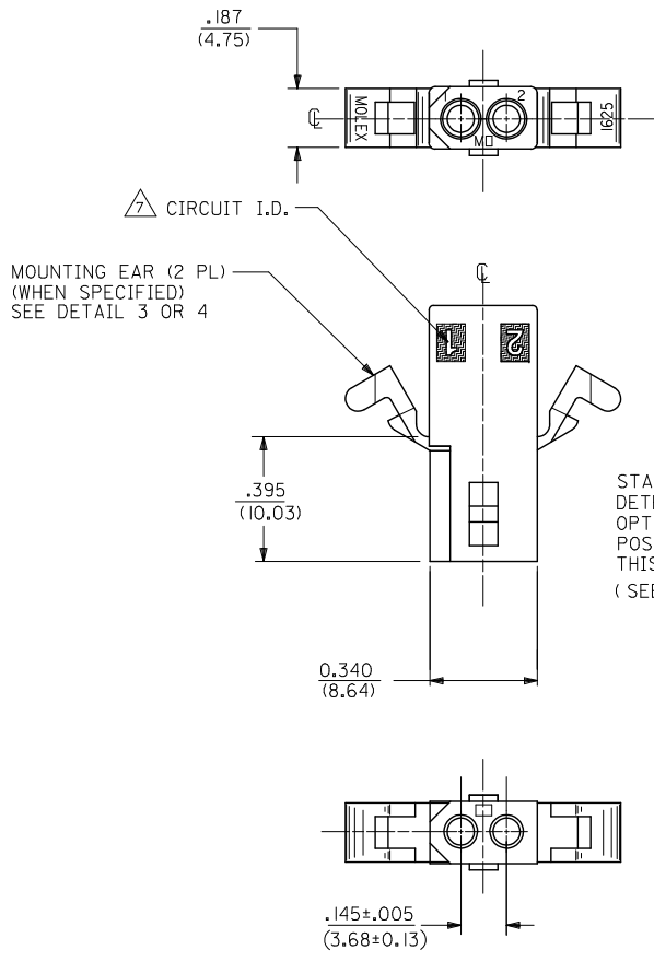
OPTIONAL POSITIVE LOCK ONE SIDE ONLY SCALE 4:1
