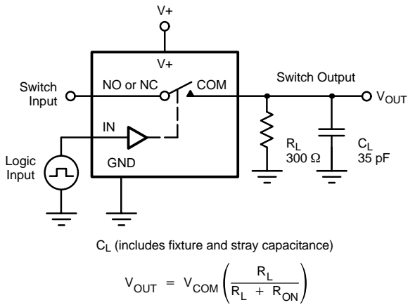
FIGURE 1. Switching Time
