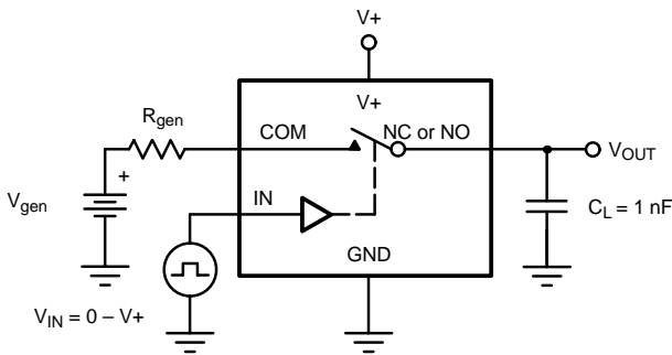
FIGURE 2. Charge Injection
