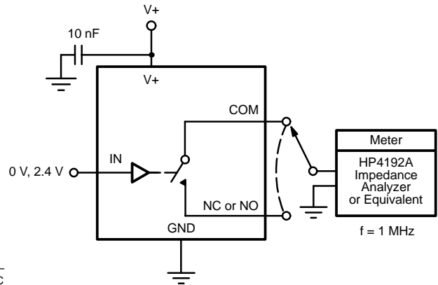
FIGURE 4. Channel Off/On Capacitance
