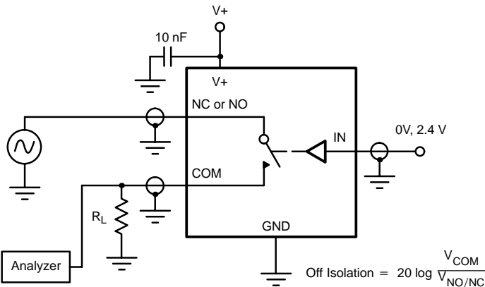
FIGURE 3. Off-Isolation
