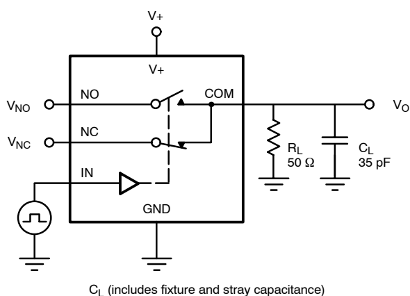
FIGURE 3. Break-Before-Make Interval
