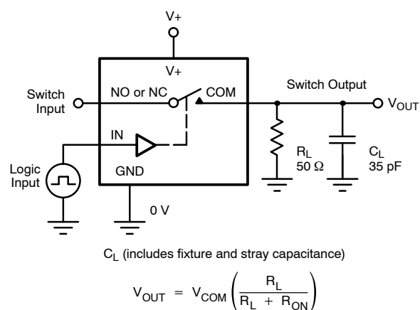
FIGURE 1. Switching Time
