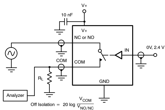
FIGURE 4. Off-Isolation
