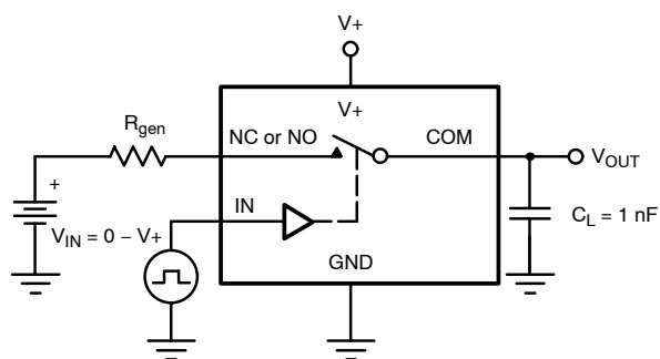
FIGURE 2. Charge Injection
